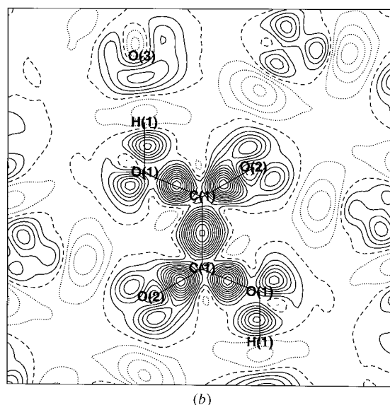
Fig. 3. Model map after multipole refinement: data cut-off at \sin \theta/\lambda = 0.9 \text{ \AA}^{-1} for reflections with F^2 > 2\sigma(F^2) ; (a) this work; (b) SC. Contour level: 0.05 e \text{ \AA}^{-3} .
